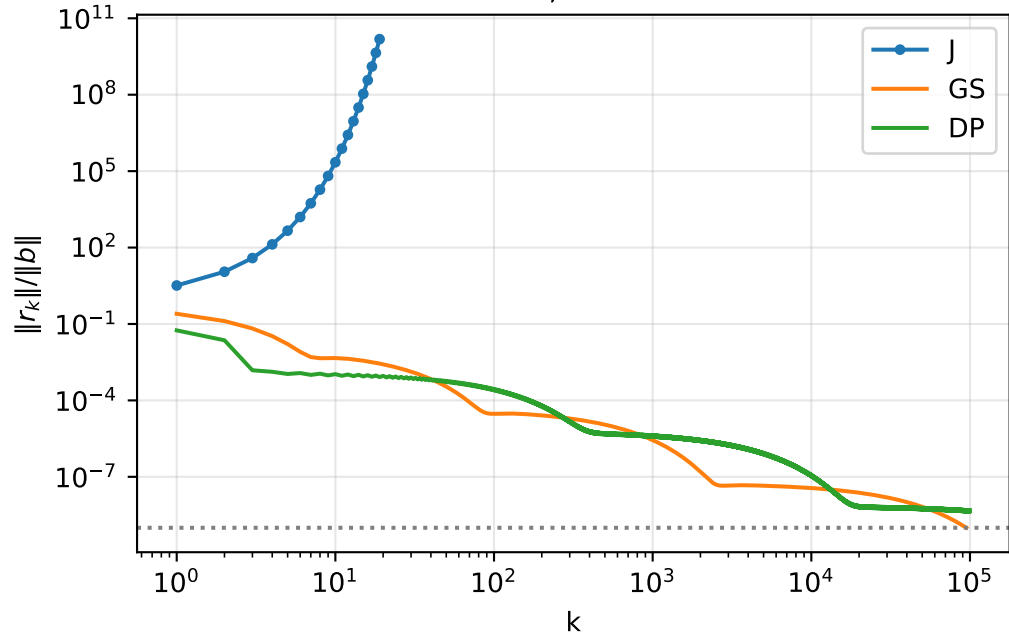
hilb, n = 5
